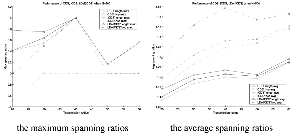
Fig. 12. The relation of the spanning ratios with the transmission radius.
