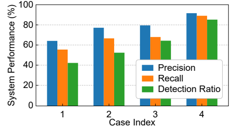
Fig. 21. Effectiveness of handling user dependence.
