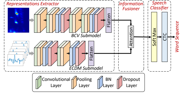
Fig. 12. The architecture of the proposed CNN-CTC model.
