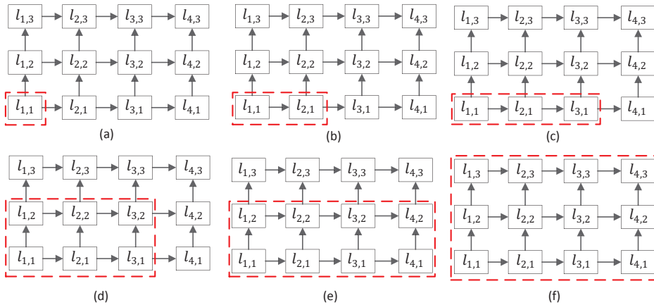
Figure 7: Coding speed illustration, CS = (1, 2, 1) .
