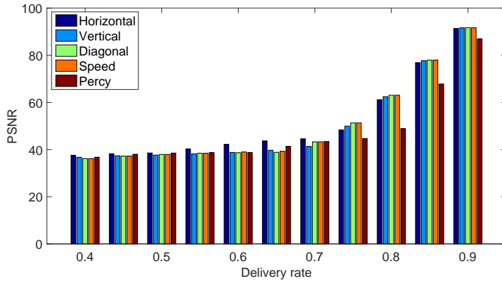
Figure 14: Akiyo video sequence [31]. PSNR of the decoded video in the case of single user. m = 4 , n = 3 , X = 20 , CS = 1 .
