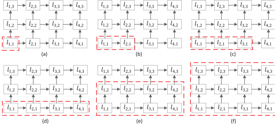
Figure 5: Horizontal Triangular Network coding scheme.
