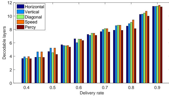
Figure 11: Number of decodable layers in the case of single user for any video. m = 4 , n = 3 , X = 15 , CS = 1 .
