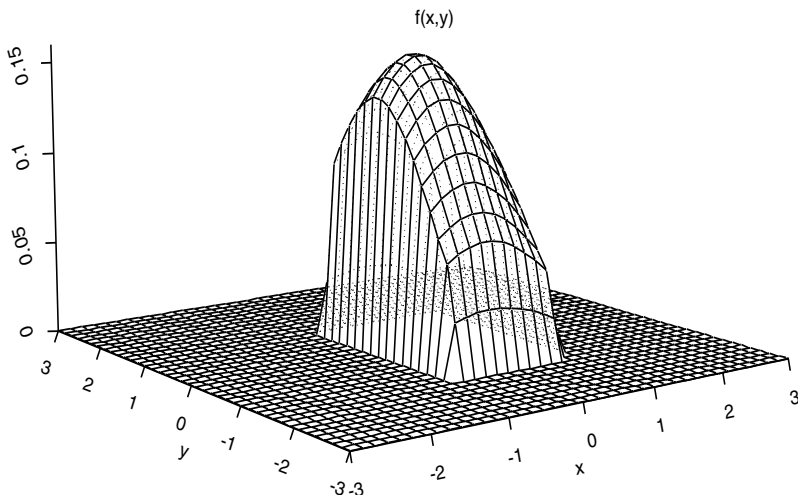
Fig. 9.1. Volume under a joint probability density function f on the rectangle [-0.5, 1] \times [-1.5, 1] .
