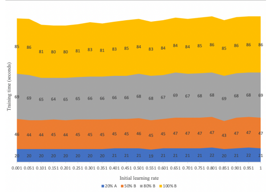
Fig. 7: Training speed of transfer A to different proportions of B, over different initial learning rates.
