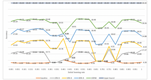
Fig. 8: Test accuracies that correspond to the training speed measured in Fig 9
