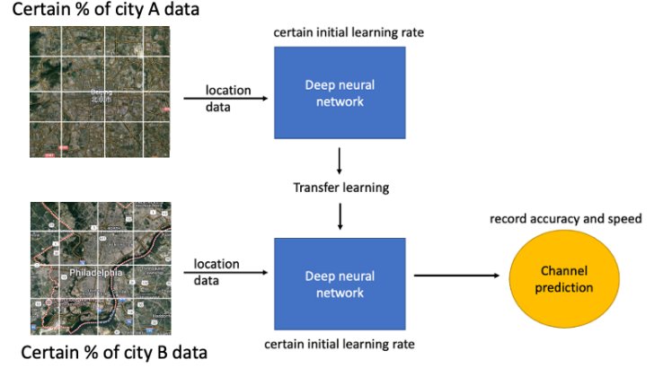
Fig. 4: Transfer learning strategy for simulations.
