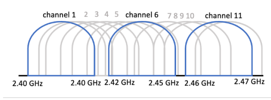
Fig. 3: Wireless channels overlap in RF frequency band.
