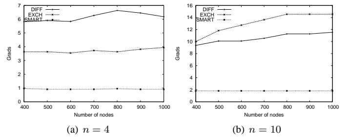
Fig. 11. Balance degree of DIFF, EXCH, and SMART by Grads ( \sigma = 1 ).
