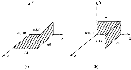
Figure 3. Planer-adaptive routing
