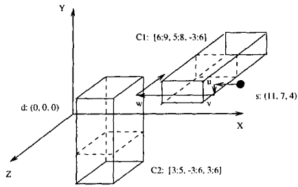
Figure 2. A routing example.
