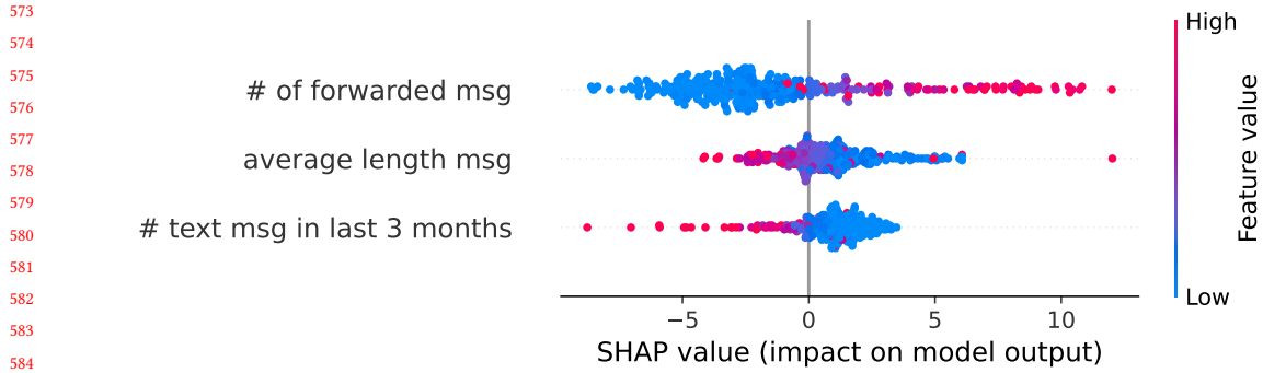
Fig. 5. SHAP values of the 3 most contributing features.
