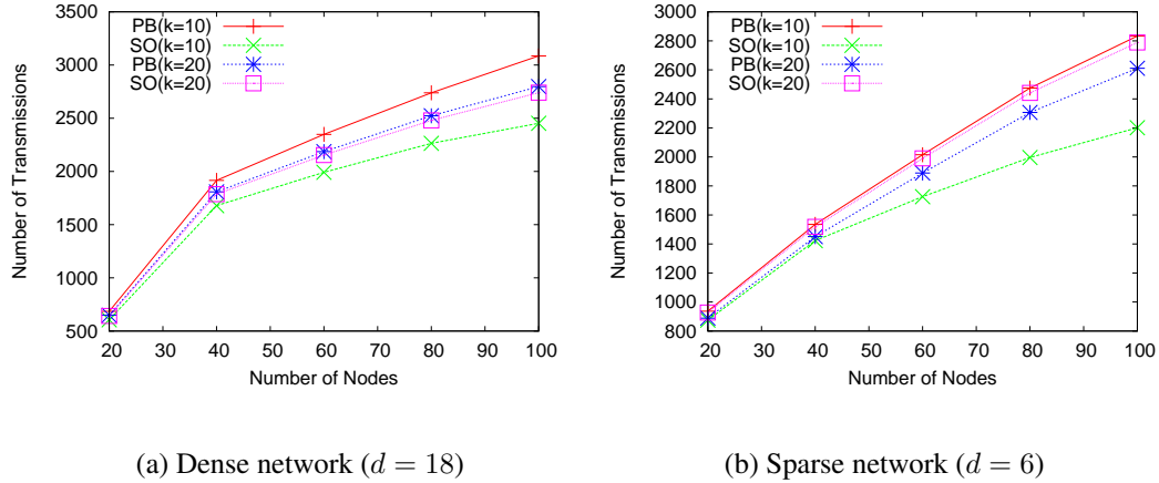
Figure 13: Comparison of PB and SO in number of transmissions.
