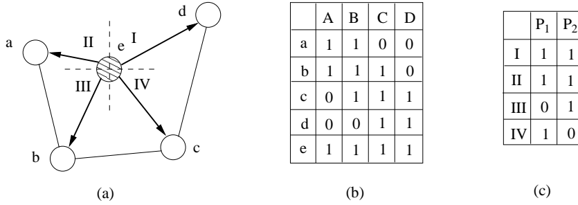
Figure 1: (a) A sample network, (b) neighbor reception table of node e , and (c) transmission table of node e using coding and directional antennas.
