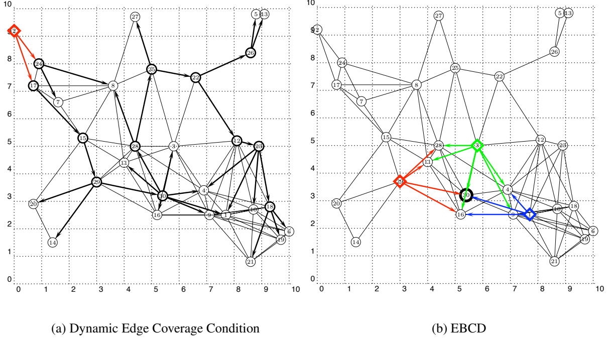
Figure 4: Examples of Dynamic Edge Coverage Condition and EBCD.
