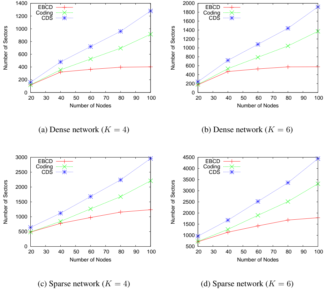
Figure 11: Comparison of EBCD, Coding, and CDS in energy consumption.
