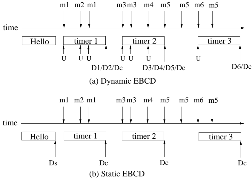
Figure 8: Illustration of execution procedure of dynamic/static EBCD.
