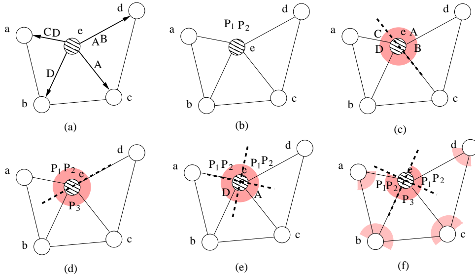
Figure 7: (a) DDCDS, (b) coding, (c) and (d) K = 2 , (e) and (f) K = 4 .
