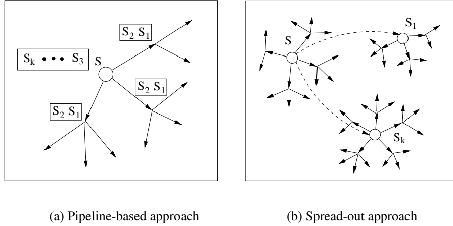
Figure 9: Single source/single message broadcast.
