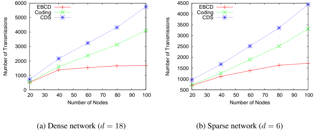
Figure 10: Comparison of EBCD, Coding, and CDS in number of transmissions.
