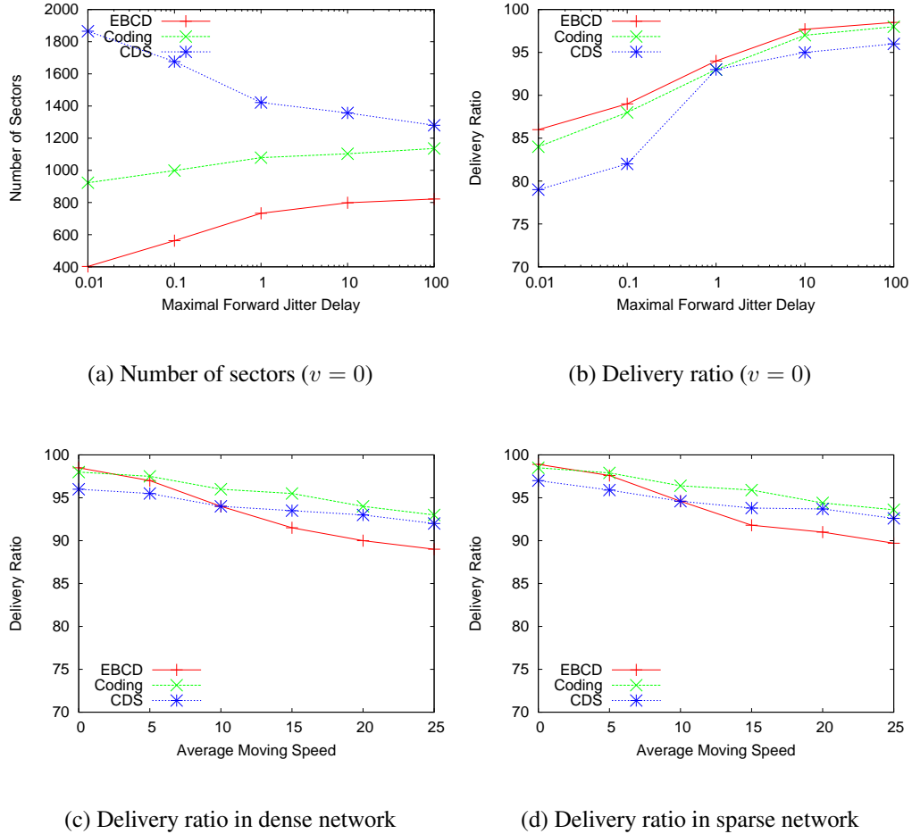
Figure 14: Performance in dynamic environment with collision and mobility ( K = 4, n = 100 ).
