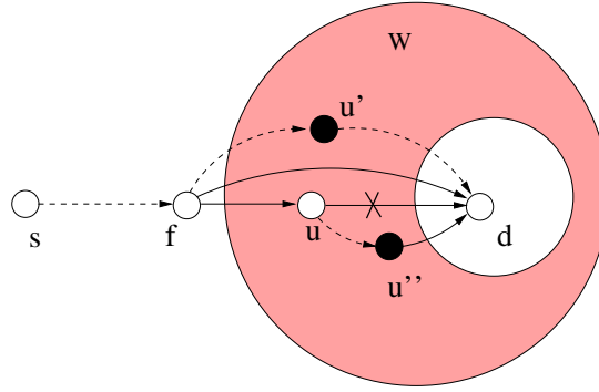
Figure 5: Proof of dynamic node/edge coverage conditions.
