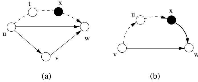
Figure 3: Directed replacement paths in (a) node coverage, and (b) edge coverage with visited nodes.
