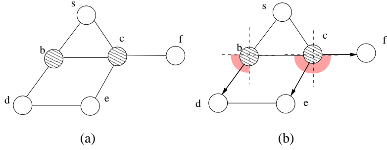
Figure 6: (a) Forward nodes, (b) forwarding nodes and forwarding edges.
