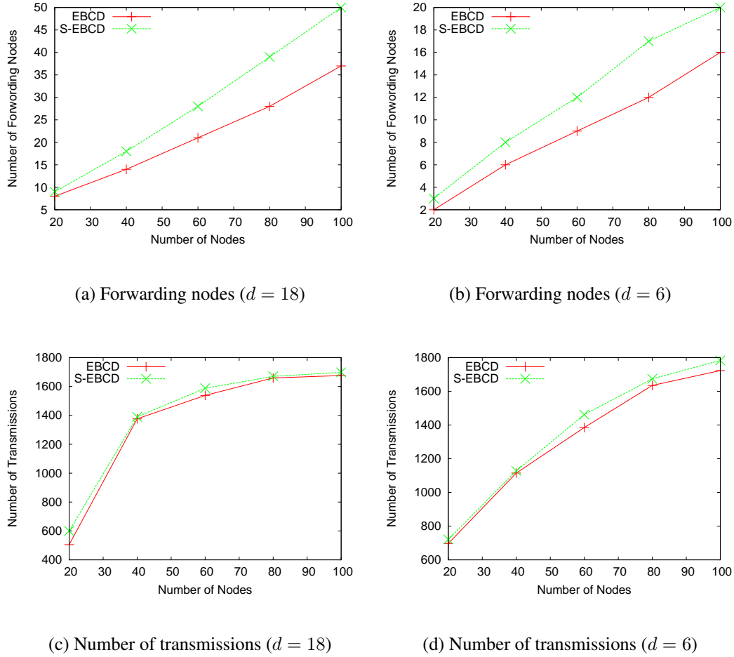
Figure 12: Comparison of EBCD and S-EBCD.
