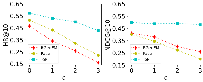
Fig. 7. Comparison of short-term ( t_c, c = 0 ) and long-term ( t_c, c = 1, 2, 3 ) POI recommendations with baselines.
