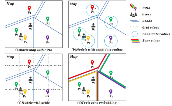
Fig. 4. (a) is the basic map with POIs. (b) (c) indicate the limitations of traditional POI recommendations. In (b), for u_1 , no POI is selected as his candidates; for u_2 , models are confused by choosing p_3 or p_4 for u_2 . In (c), models ignore the road network between grids. In (d), we consider the road network and recommend POIs with different zone effects (different edge colors).
