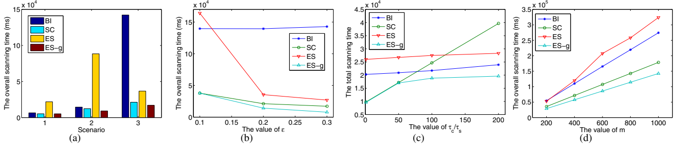
Fig. 2. Simulation results in basic histogram collection: (a)The overall scanning time in various scenarios;(b)The overall scanning time with various \epsilon ;(c)The overall scanning time with various \tau_c/\tau_s ;(d)The scanning time with various value of m .
