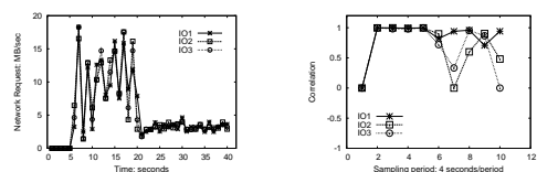
(a) External I/O request rate (b) corr(req, mem)
