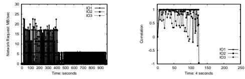
(a) External I/O request rate (b) corr(req, mem)
