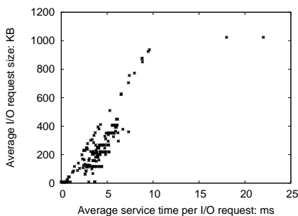
Figure 7: The relation between average I/O request size and average service time per I/O request. Data is from a trace of 250 seconds I/O activities on a computer node.
