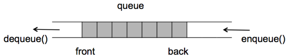
Figure 7.1: Queue
