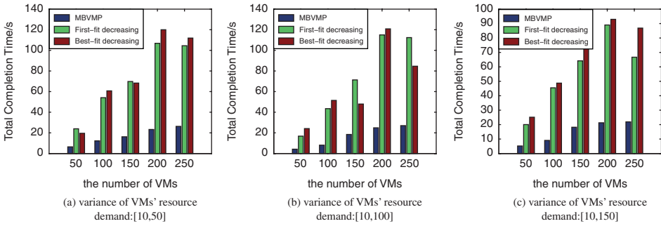
Figure 8. Performance comparisons of total completion time versus variance of VMs' resource demand.
