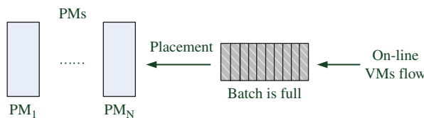
Figure 4. Provider-oriented batch.
