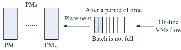
Figure 5. User-oriented batch.
