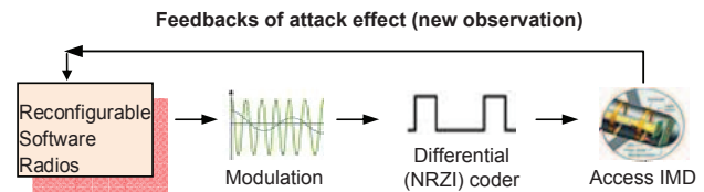
Fig. 1. Launching RD attacks using software radios
